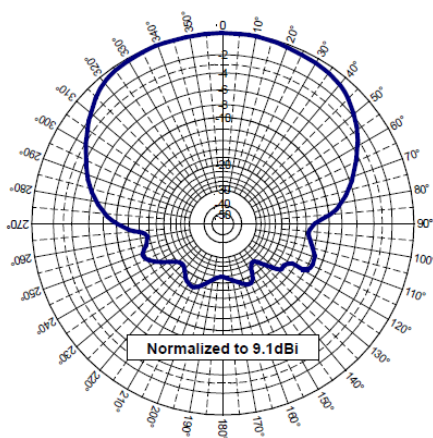
Elevation Pattern ( \Phi = 90^\circ )
