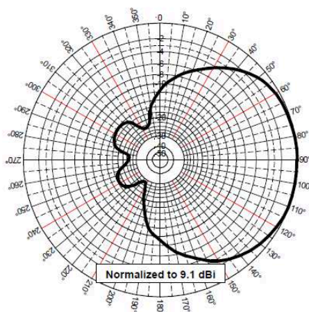
Azimuthal Pattern ( \Phi = 0^\circ )
